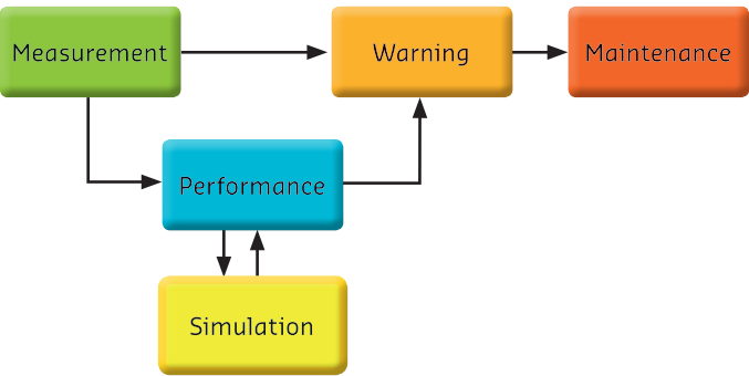
Performance monitoring through coupling with SCADA system
