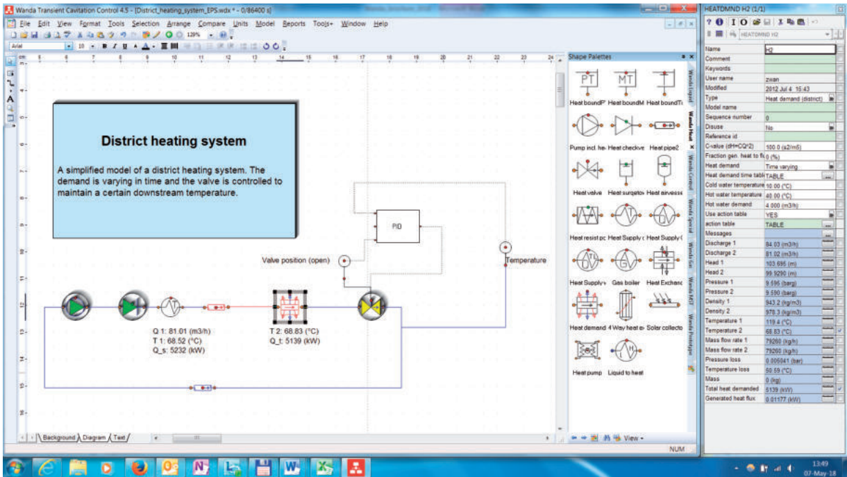
Modelling a district heating system in WANDA
