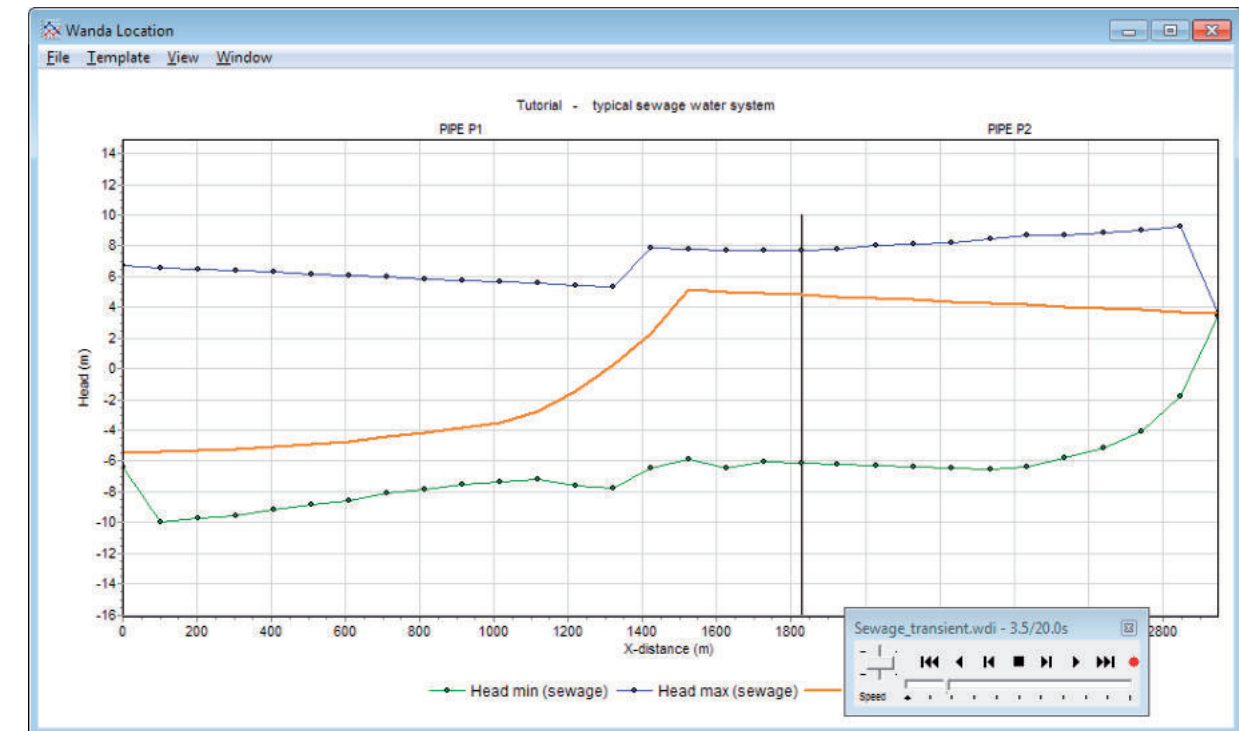
Analysis of pressure wave propagation through a pipeline
