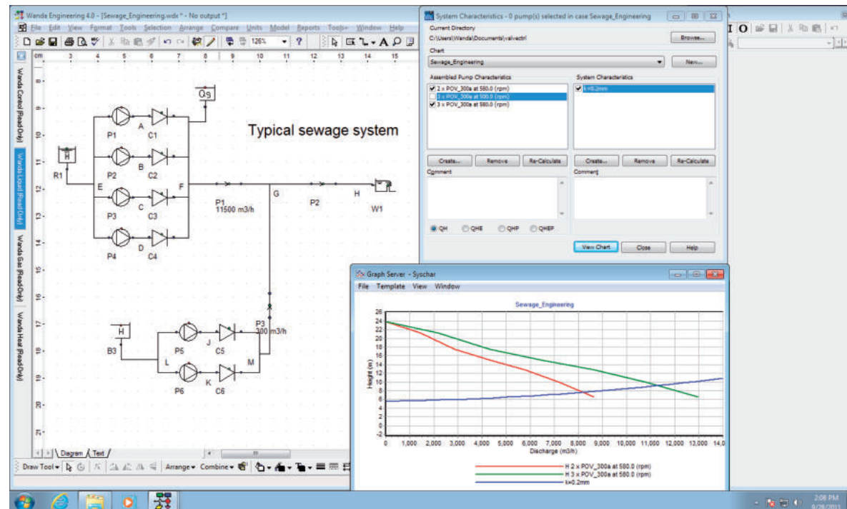
Hydraulic design of a pipeline system
